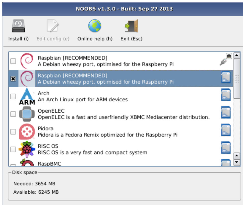
Figure 1.5 Selecting Raspbian
